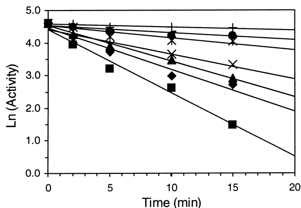
Figure 2. Inactivation of caspase-3 (250 ng/mL, 200 μL) with N -nitrosoanilines (5 mM, 200 μL) in 10 mM Tris buffer (pH 7.5, 1 mM EDTA). Pseudo-first order rate constants (min -1 ): 3 (◆ 0.129); 4 (■ 0.195); 5 (▲ 0.109); 6 (× 0.076); 7 (* 0.038); 8 (● 0.023); 9 (+ 0.009); 10 (– 0.023). Trendline of 10 overlaps with that of 8.
