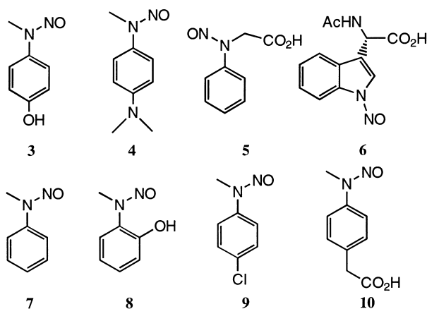
Figure 1. Non-peptide based N -nitroso compounds.
