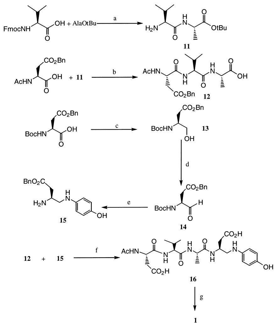
Figure 4. Synthetic approach toward inhibitor 1. (a) (i) EDC, HOBT/CH 2 Cl 2 ; (ii) Et 3 NH, DMF; (b) (i) EDC, HOBT/CH 2 Cl 2 ; (ii) TFA, CH 2 Cl 2 ; (c) (i) t -BuOCOCl, NMM, TFA; (ii) NaBH 4 , MeOH, THF; (d) (COCl) 2 , DMSO, Et 3 N, CH 2 Cl 2 ; (e) (i) 4-aminophenol, NaCNBH 3 , MeOH; (ii) TFA, DCM; (f) (i) EDC, Et 3 N, CH 2 Cl 2 ; (ii) H 2 /Pd-C; (g) NaNO 2 , HCl/H 2 O.
