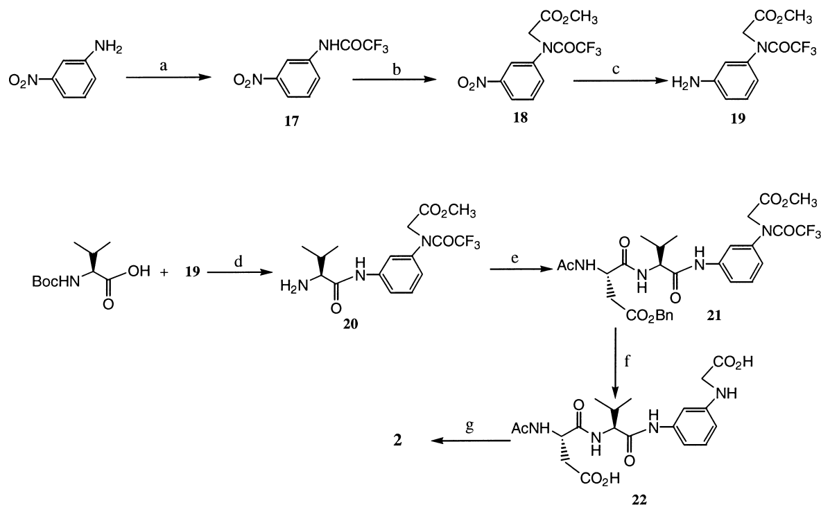
Figure 5. Synthetic approach toward inhibitor 2 . (a) 1.1 equiv (\text{COCF}_3)_2\text{O} ; (b) \text{BrCH}_2\text{COOCH}_3 , NaH, DMF; (c) \text{RaNi} , 2-propanol; (d) (i) EDC, \text{CH}_2\text{Cl}_2 ; (ii) DMAP, DMF; (iii) 3 M HCl in EtOAc; (e) Ac-Asp- \beta -(OBn), EDC, Pyr; (f) (i) \text{K}_2\text{CO}_3 , MeOH/ \text{H}_2\text{O} ; (ii) KOH; (g) \text{NaNO}_2 , HCl/ \text{H}_2\text{O} .
