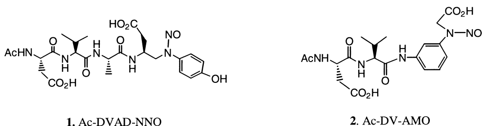
Figure 3. Structures of Ac-DVAD-NNO (1) and Ac-DV-AMO (2).
